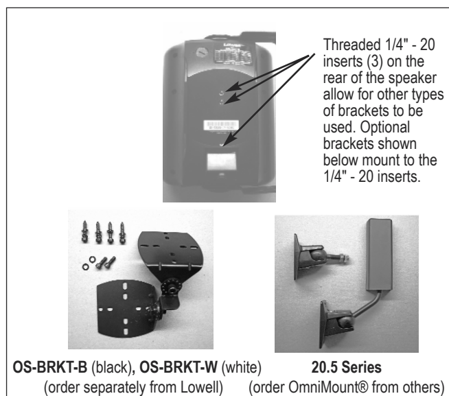
Installation using optional brackets
