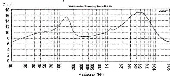
Impedance - 8ohm
