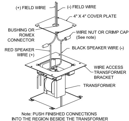
(Fig. 1) Typical wiring diagram.
