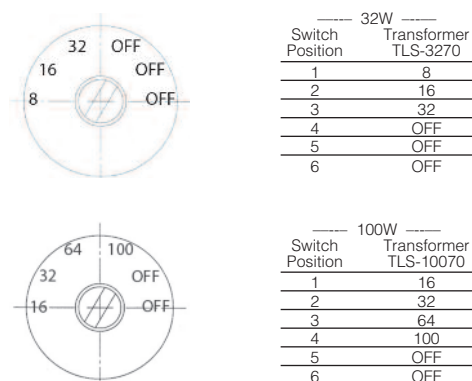
(Fig. 3) Transformer power tap settings.
