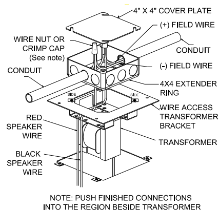
(Fig. 2) Wiring diagram when in/out conduit is specified.
