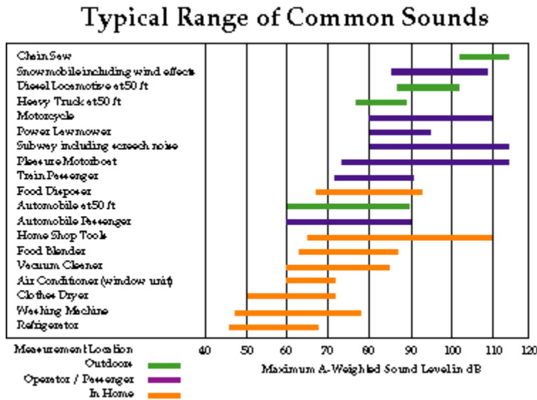
Fig. 1 - Typical Range of Common Sounds
